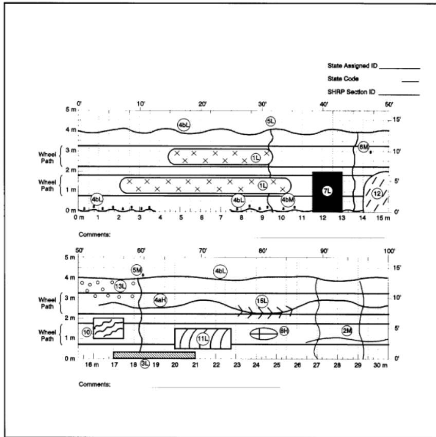
Figure 1: Example distress survey map for asphalt pavement
