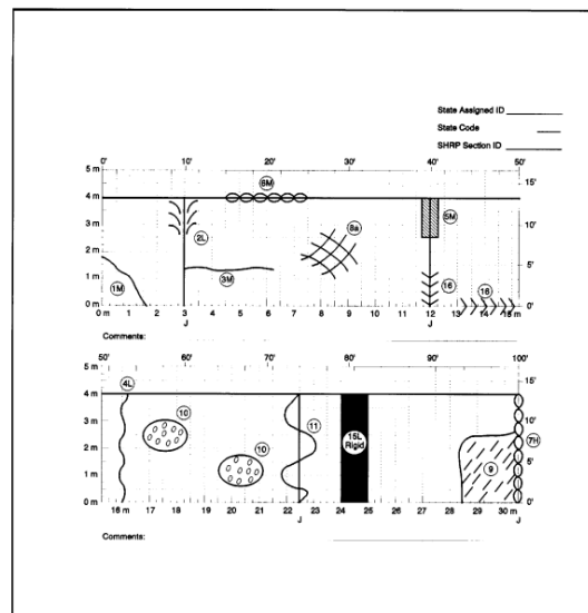
Figure 2: Example distress survey map for jointed concrete pavement
